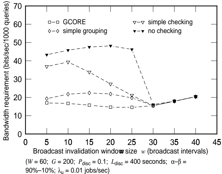
Figure 9: Impact of broadcast invalidation window size.
