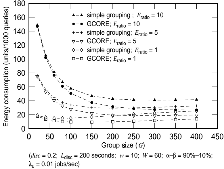
Figure 15: Impact of group size on energy consumption.
