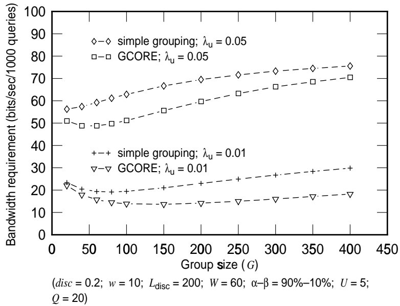
Figure 13: Impact of group size on bandwidth.
